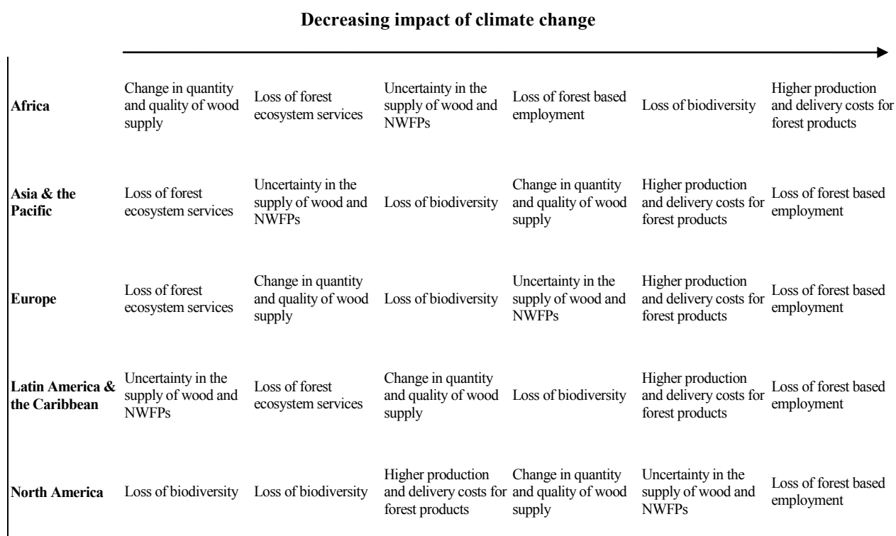
Figure 3. Future impacts of climate change on forests and people
