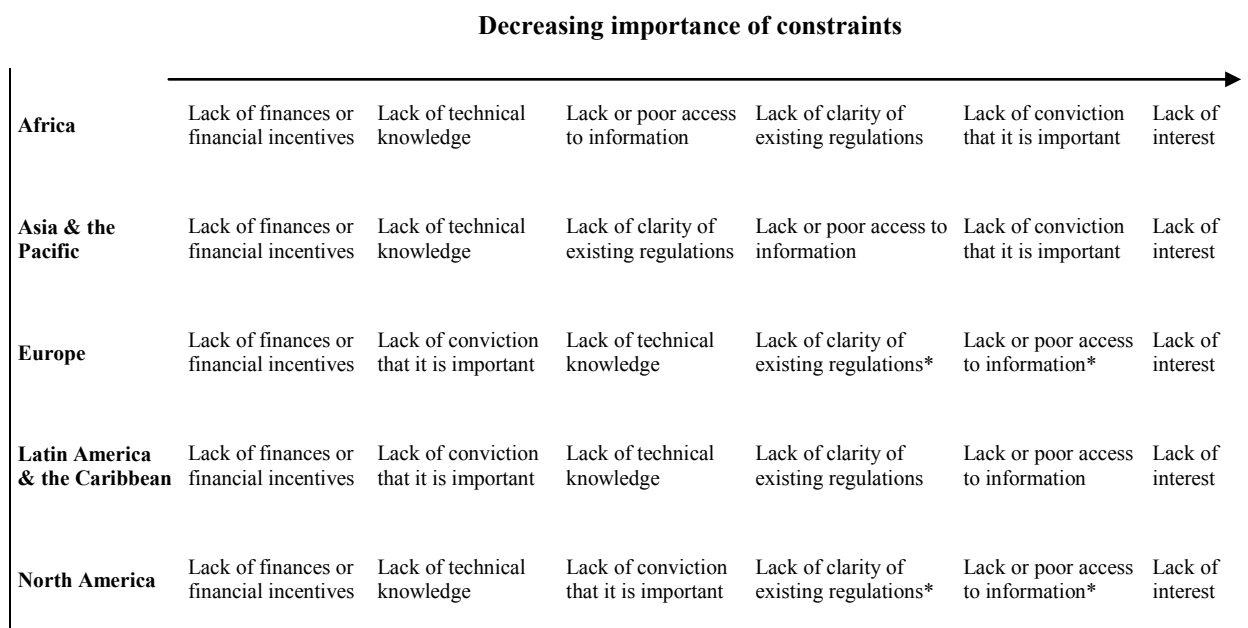
Figure 6. Constraints limiting climate change adaptation and mitigation actions
