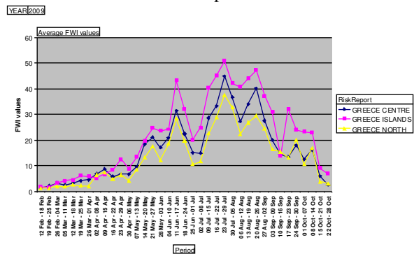
Figure 59. Fire danger trends in 2009 as determined by the Fire Weather Index (FWI) in the regions identified for Greece
