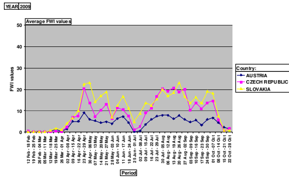
Figure 64. Fire danger trends 2007-2009 in some EU temperate countries (AT, CZ, SK).
