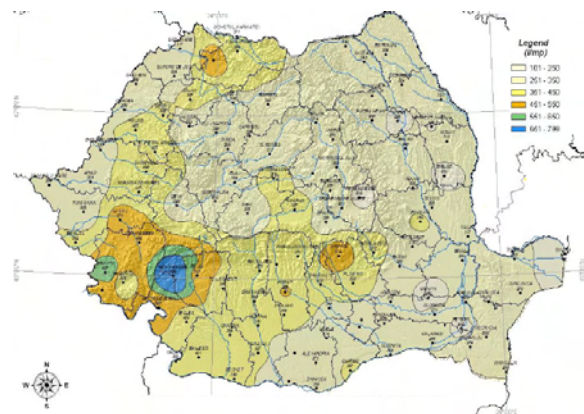
Figure 36. Precipitations recorded between September 2008 and May 2009
