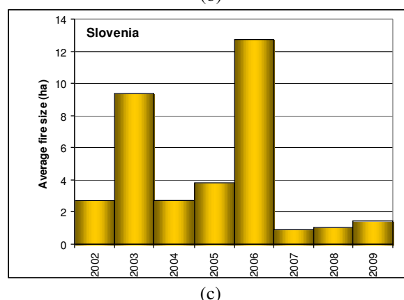
Figure 44. Burnt areas (a), number of fires (b) and average fire size (c) in Slovenia from 2002 to 2009
