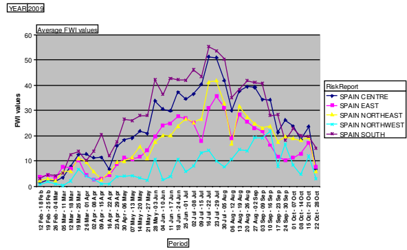
Figure 58. Fire danger trends in 2009 as determined by the Fire Weather Index (FWI) in the regions identified for Spain
