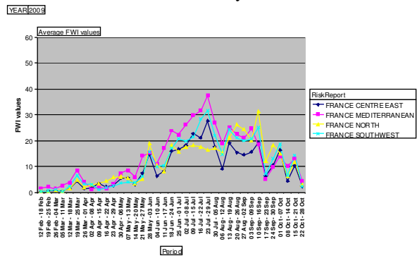
Figure 61. Fire danger trends in 2009 as determined by the Fire Weather Index (FWI) in the regions identified for France.
