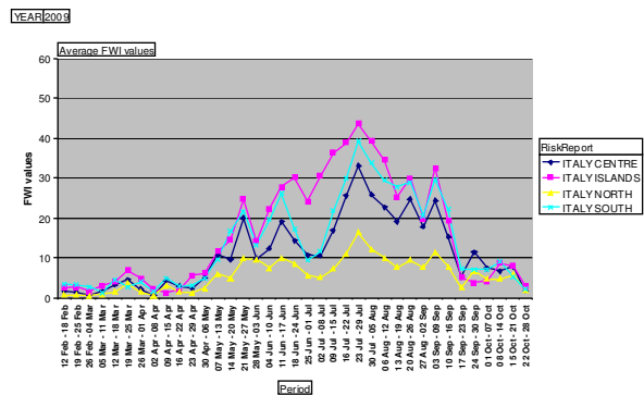
Figure 60. Fire danger trends in 2009 as determined by the Fire Weather Index (FWI) in the regions identified for Italy
